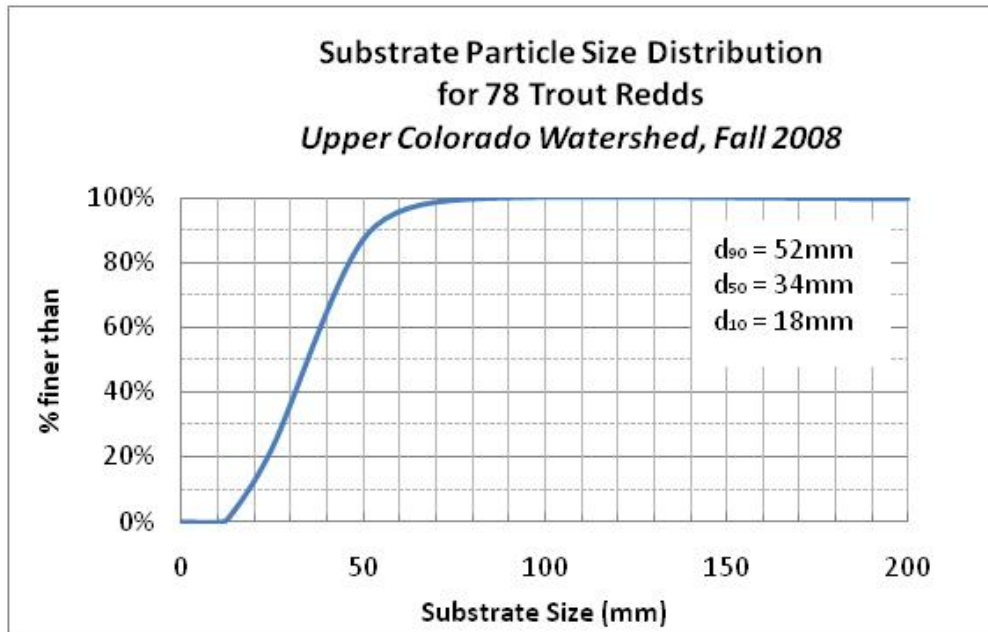
Figure ES-4. Substrate Particle Size Distribution Plot
