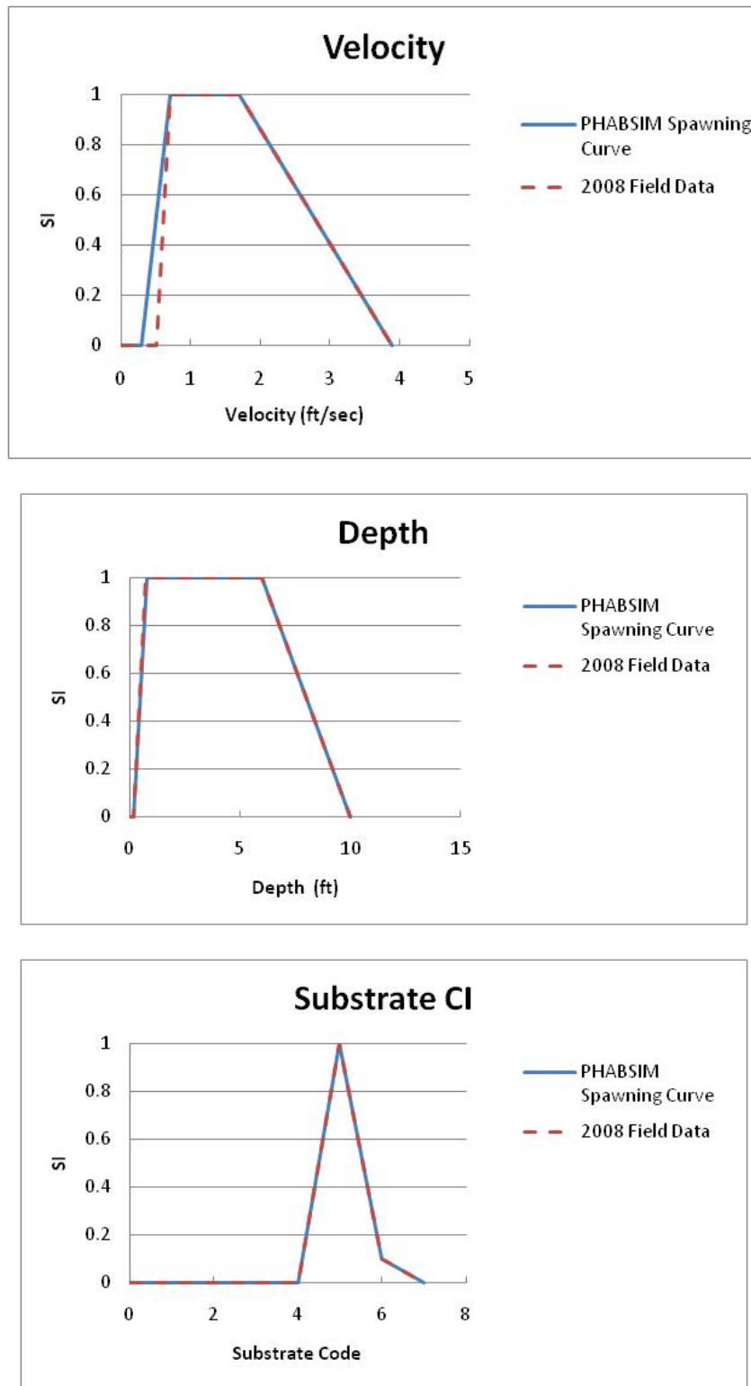
Figure ES-3. Spawning Suitability Curves The velocity, depth and substrate channel index (CI) spawning suitability curves used for the PHABSIM studies as compared to trout redd data collected in Fall 2008.
